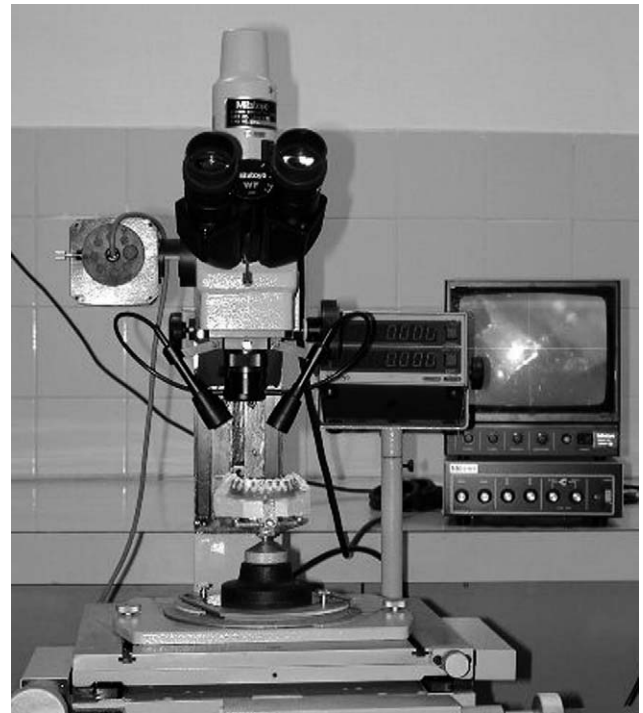
Figure 2. A setup model is placed in a toolmaker's microscope for measuring RotD in millimeters.
